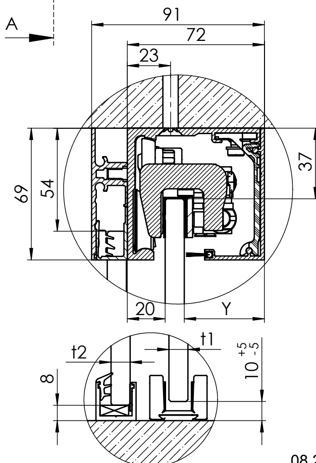
Detail X (1 : 2)
